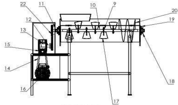
VISTA FRONTAL
